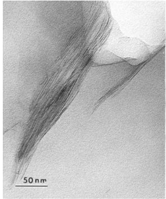
Figure 8. TEM of DMHDIM-MMT/PS (95:5)
