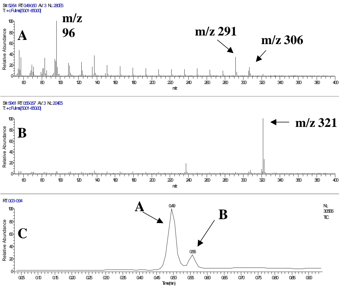
Figure 5. Thermal desorption electron ionization mass spectrum of DMHDIM + Cl - (C) and total ion plot of the peaks at 0.49 min (A) and 0.55 min (B).
