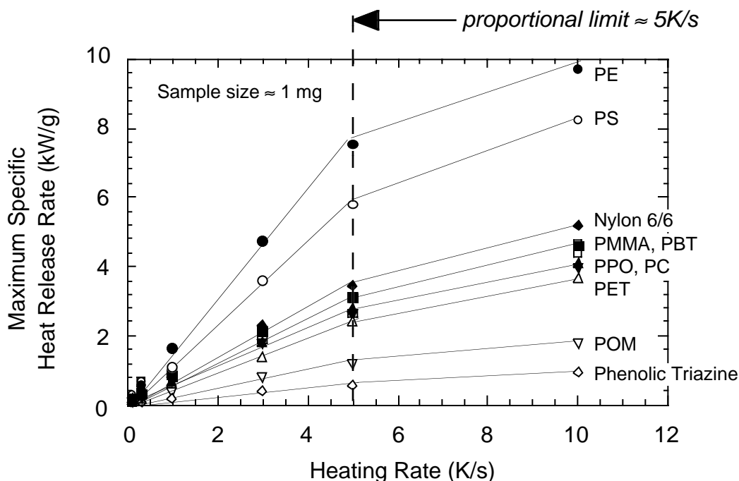
FIGURE 7. SPECIFIC HEAT RELEASE RATE VERSUS HEATING RATE FOR 1-milligram SAMPLES OF SEVERAL COMMON POLYMERS
