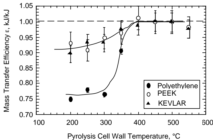
FIGURE 3. EFFECT OF PYROLYSIS CELL WALL TEMPERATURE ON MASS TRANSFER EFFICIENCY OF PYROLYSIS GASES FOR PEEK, KEVLAR™, AND POLYETHYLENE
