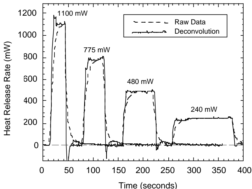
FIGURE 5. HEAT RELEASE RATE SIGNAL FOR SQUARE WAVE METHANE CALIBRATION PULSES BEFORE AND AFTER SIGNAL DECONVOLUTION
