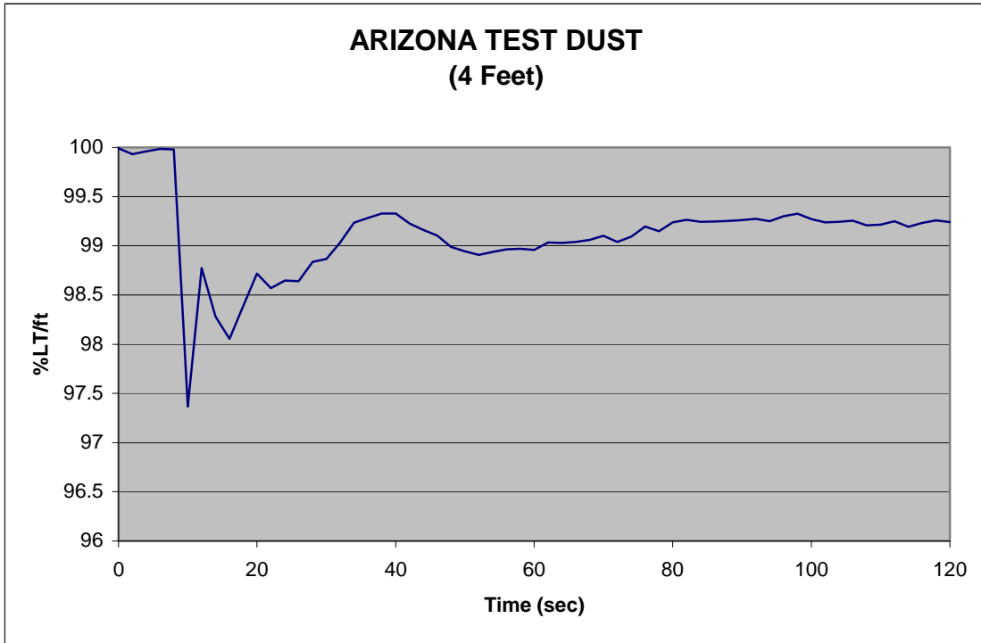
Figure 62. Arizona Test Dust Percent Light Transmission per Foot (4 Feet From Recessed Pan)
