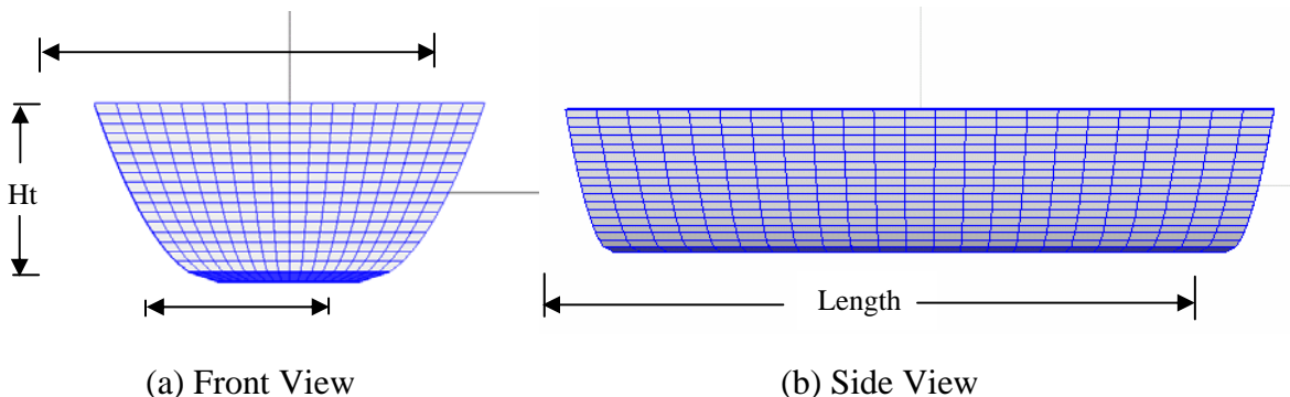
Figure 16. Computational Fluid Dynamic Model Mesh Used in Simulations
