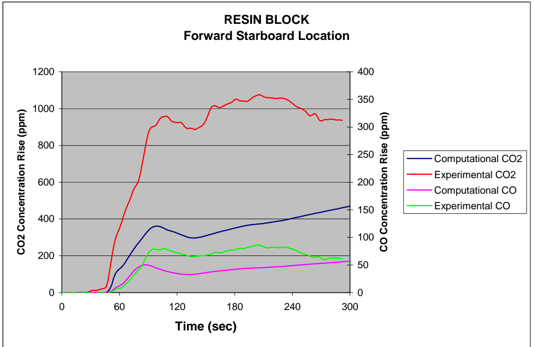
Figure 70. Comparison of Computational and Experimental Resin Block CO and CO 2 Gas Concentrations at Forward Starboard Location
