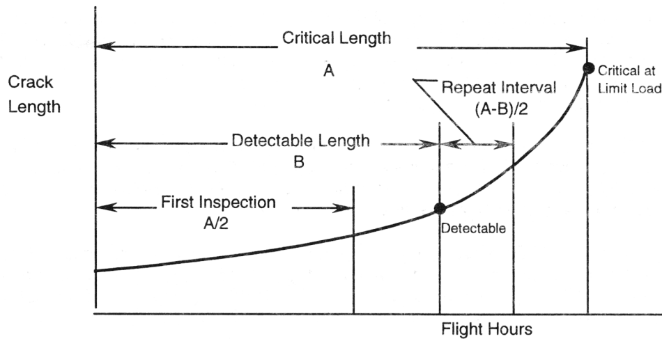
Figure 2. Typical Crack Growth Curve
