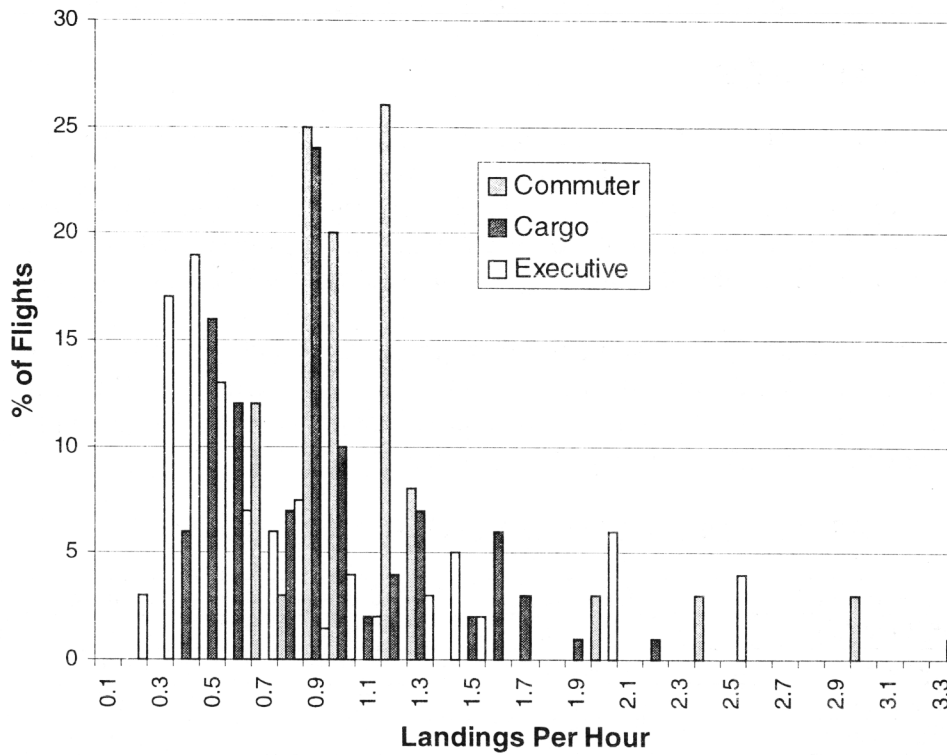
FIGURE 6. LANDINGS PER HOUR DISTRIBUTION
