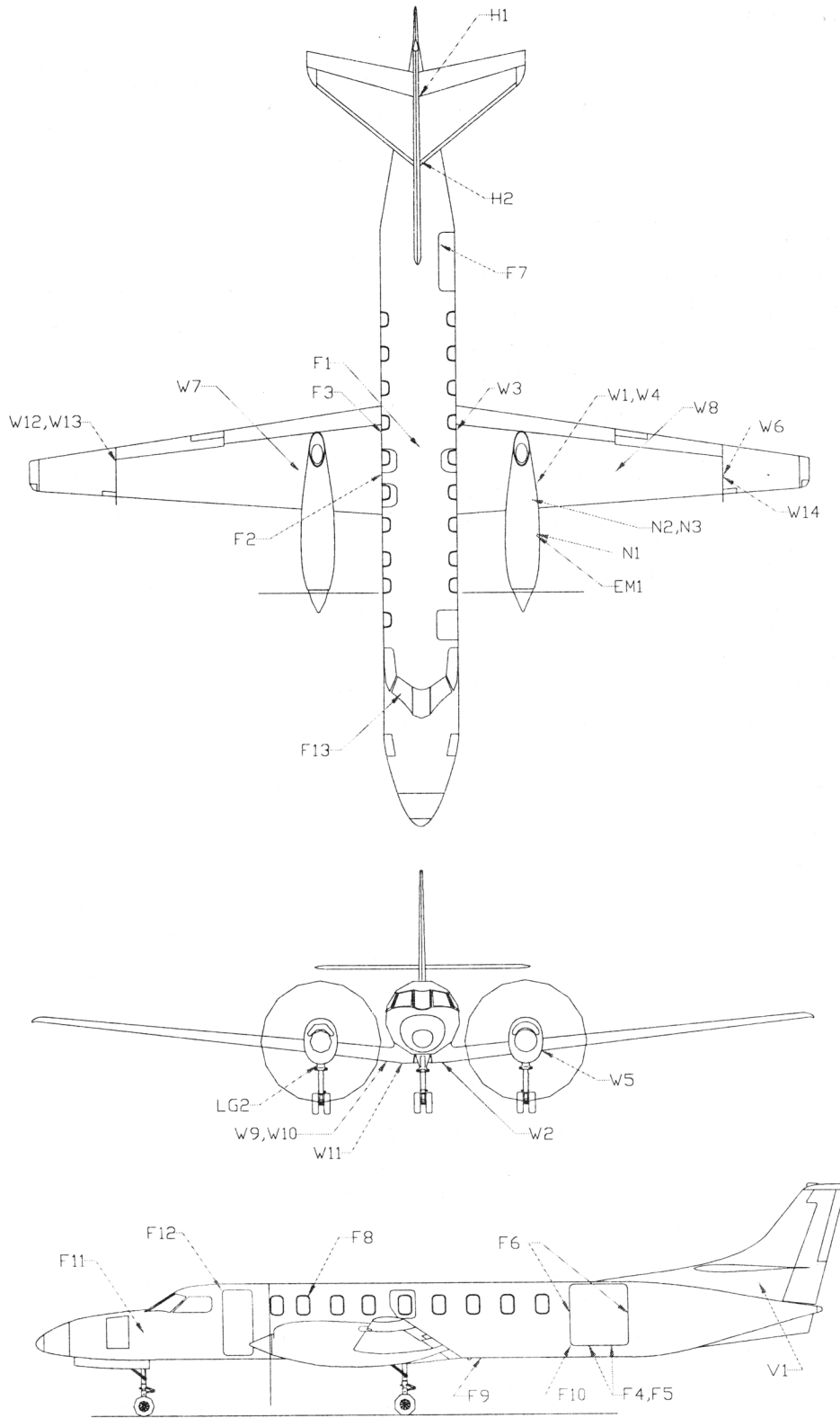
FIGURE 4. LOCATIONS OF CRITICAL AREAS
