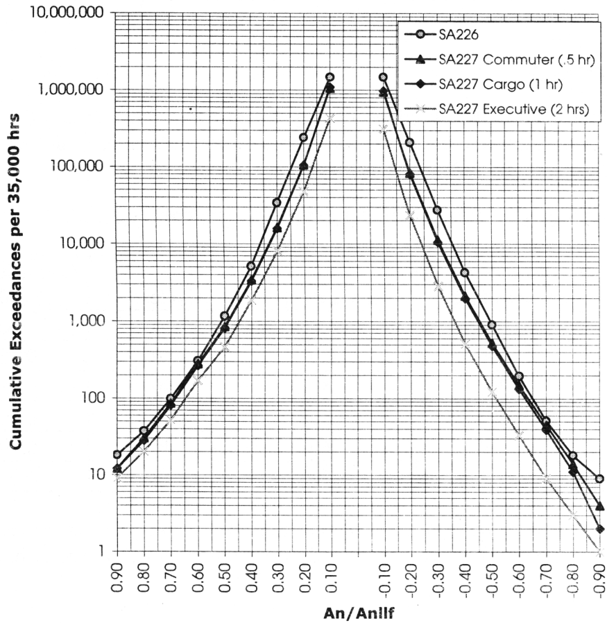
FIGURE 8. GUST AND MANEUVER LOAD SPECTRA
