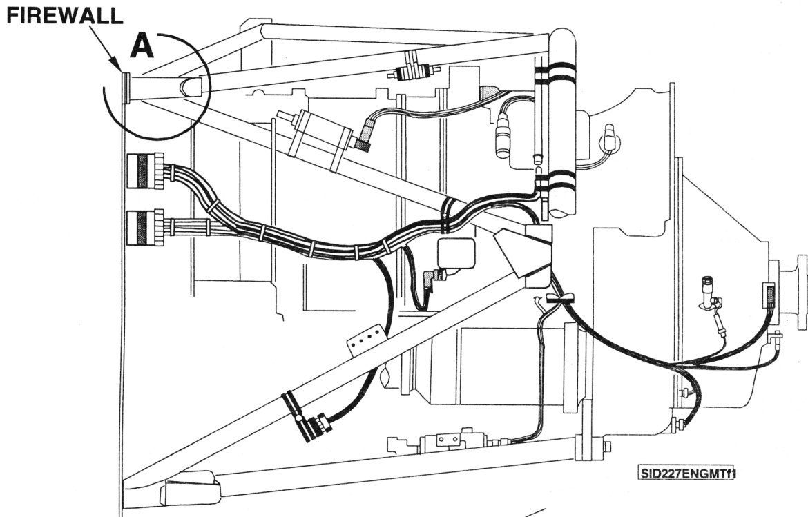
LH/RH ENGINE
