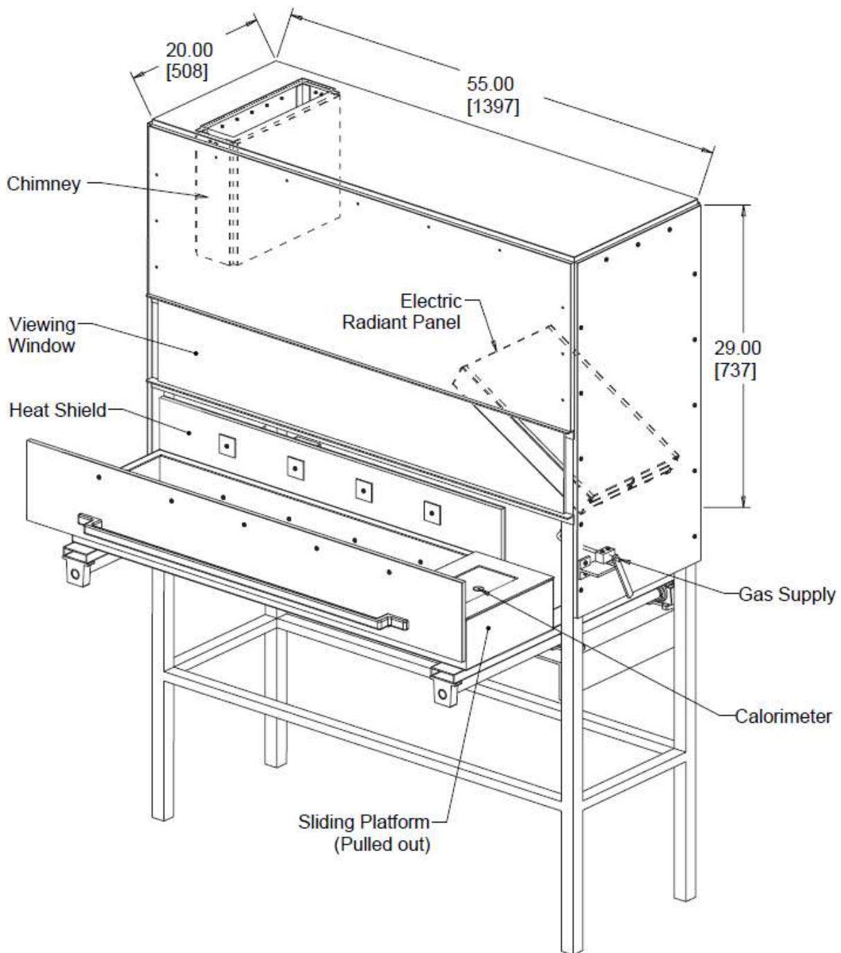
Figure 26-1. Test chamber
