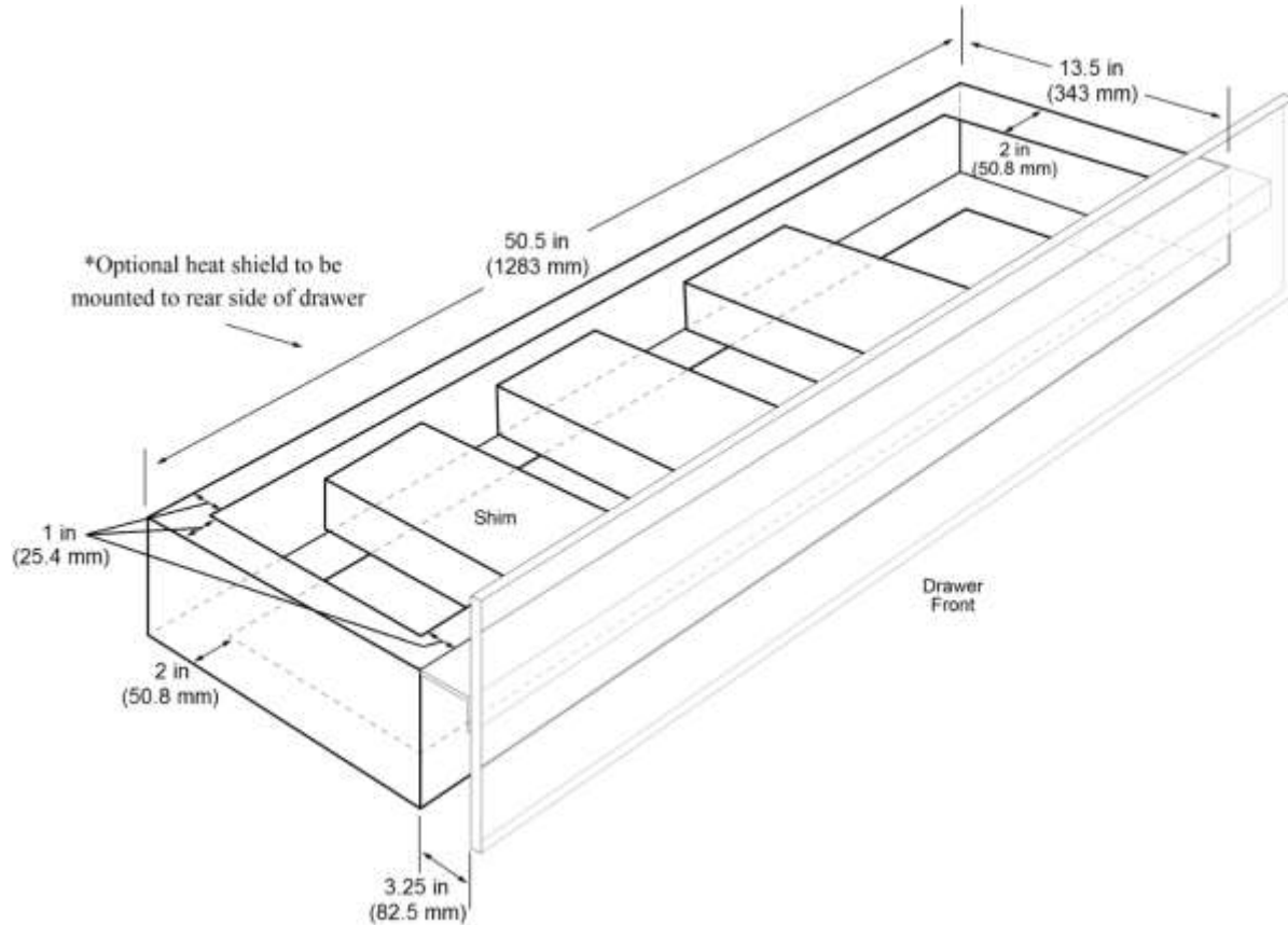
Figure 26-4. Sliding platform
