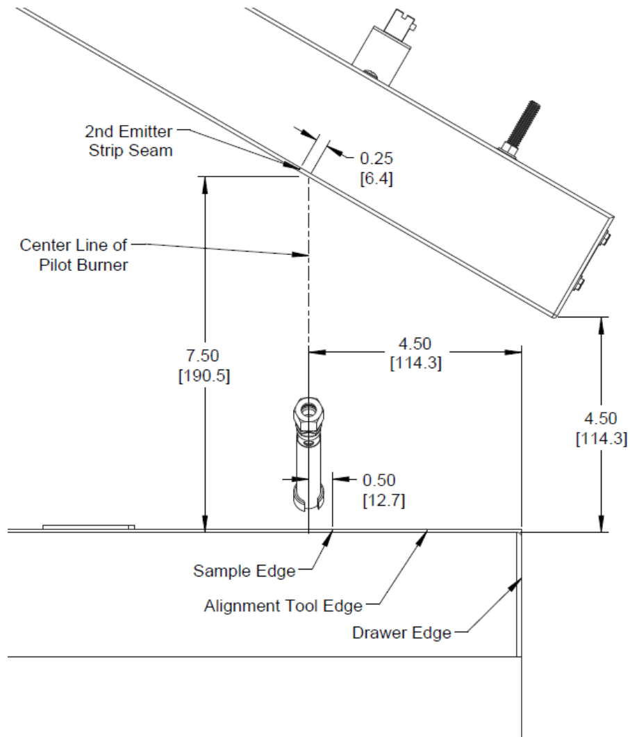
Figure 26-9. Sample holder positioning on sliding drawer
