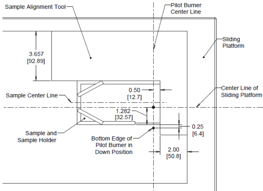
Figure 26-8. Sample holder alignment tool located on sliding drawer
