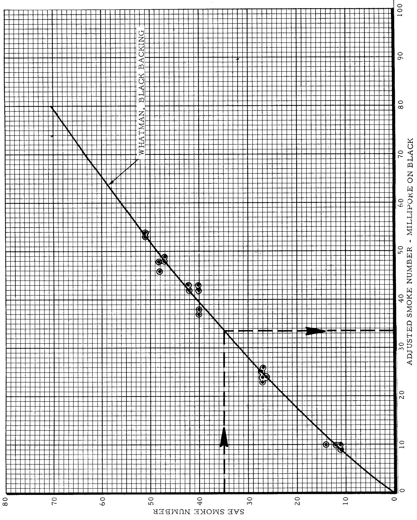
FIGURE 1 - SMOKE NUMBER ADJUSTMENT
