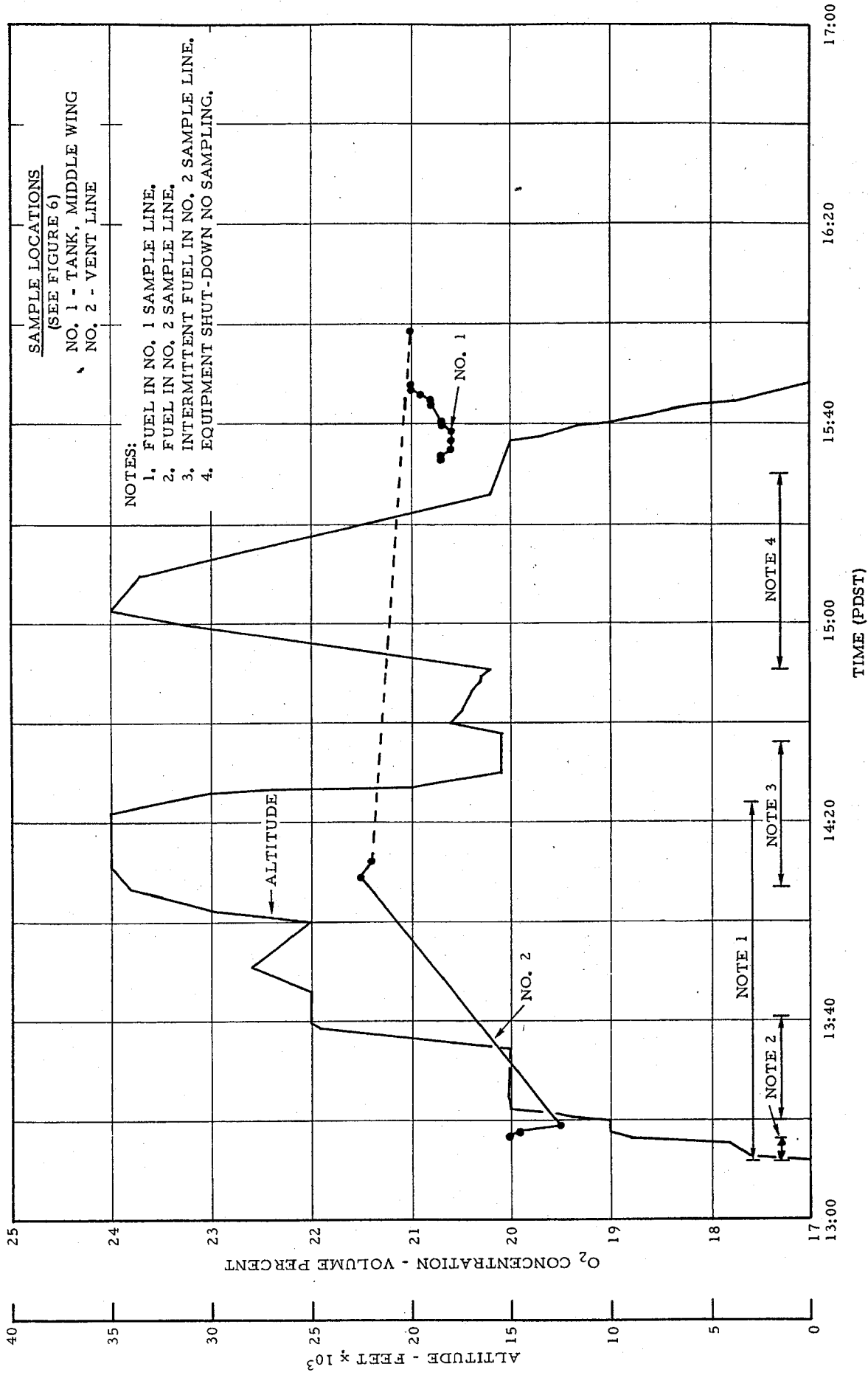
FIGURE 9 - OXYGEN CONCENTRATIONS IN LEFT MAIN FUEL SYSTEM FOR FLIGHT 1
