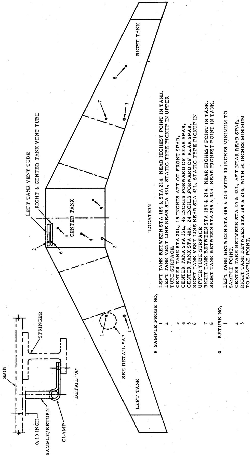
FIGURE 6 - FUEL SYSTEM VAPOR SAMPLE AND RETURN LOCATIONS
